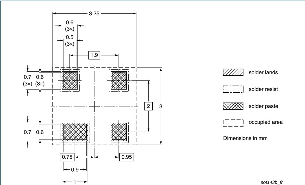
Fig 10. Reflow soldering footprint SOT143B
