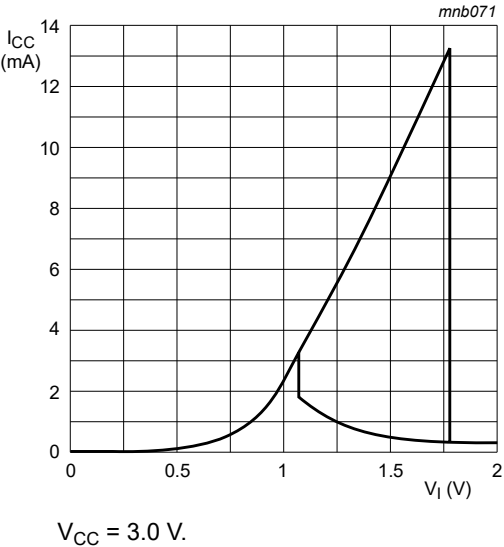
Fig. 7. Typical transfer characteristic
