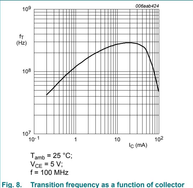
Fig. 8. Transition frequency as a function of collector current; typical values
