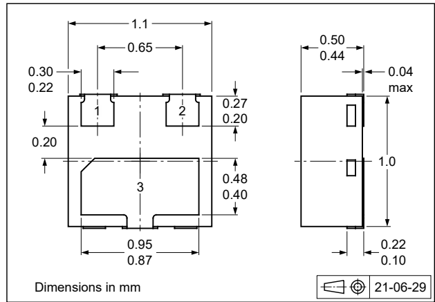
Fig. 12. Package outline DFN1110D-3 (SOT8015)
