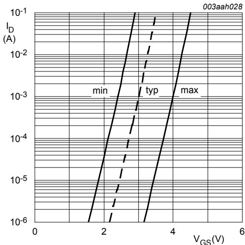
Fig. 10. Sub-threshold drain current as a function of gate-source voltage T_j = 25^\circ\text{C}; V_{DS} = 5\text{V}
