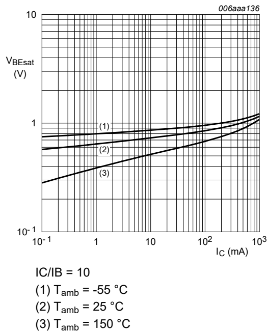
Fig. 14. BC817-40QC: Base-emitter saturation voltage as a function of collector current; typical values
