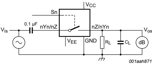
Fig. 14. Test circuit for measuring sine-wave distortion
