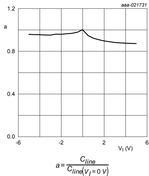
Fig. 2. Relative capacitance as a function of input voltage; typical values
