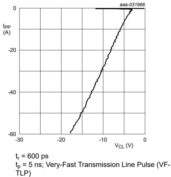
Fig. 8. Dynamic resistance with negative clamping; typical values
