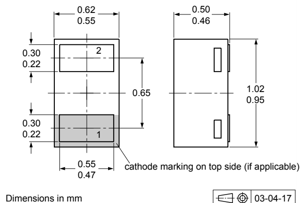
Fig. 9. Package outline DFN1006-2 (SOD882)
