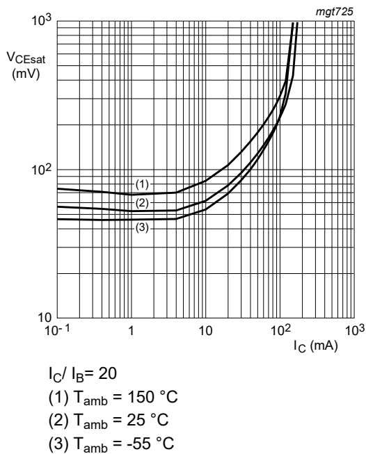
Fig. 6. BC847AQB-Q: Collector-emitter saturation voltage as a function of collector current; typical values
