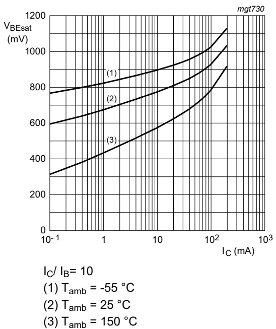
Fig. 11. BC847BQB-Q: Base-emitter saturation voltage as a function of collector current; typical values
