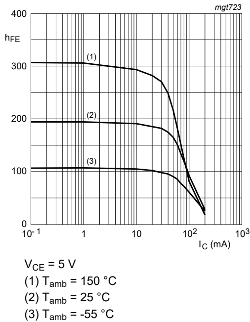
Fig. 4. BC847AQB-Q: DC current gain as a function of collector current; typical values
