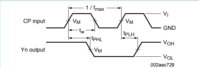
Measurement points are given in Table 8 . V_{OL} and V_{OH} are typical voltage output levels that occur with the output load. Figure 8. CP input to Yn output propagation delays, clock pulse width and maximum clock frequency
