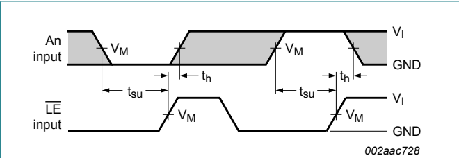
Measurement points are given in Table 8 . The shaded areas indicate when the input is permitted to change for predictable output performance. Figure 7. Data set-up and hold times, An input to LE input
