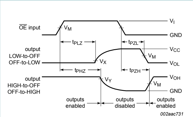
Measurement points are given in Table 8 . V_{OL} and V_{OH} are typical voltage output levels that occur with the output load. Figure 10. 3-state enable and disable times
