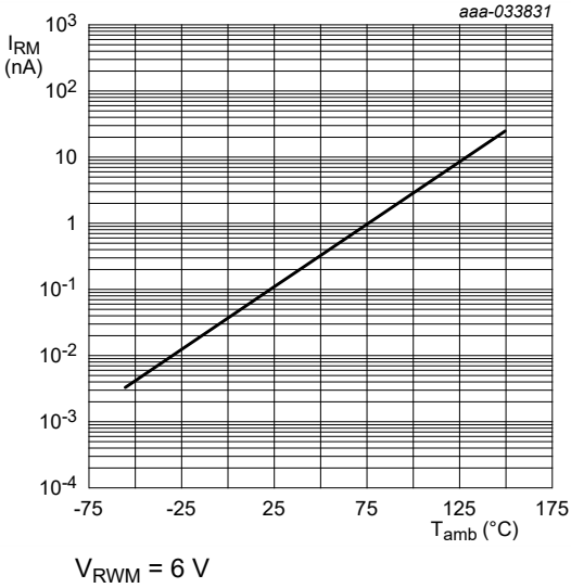
Fig. 6. Reverse leakage current as a function of ambient temperature; typical values
