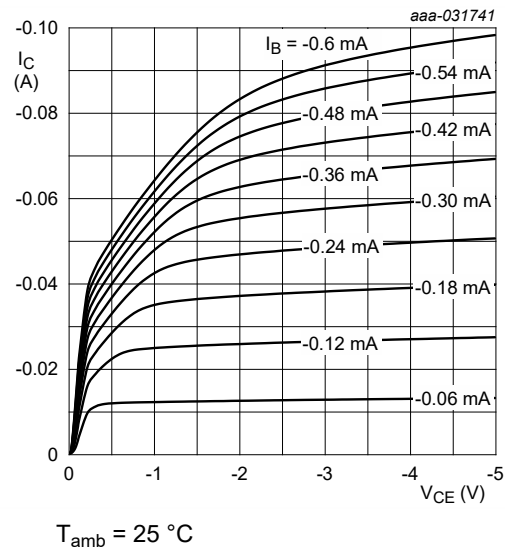
Fig. 5. NHDTA123JT: Collector current as a function of collector-emitter voltage; typical values
