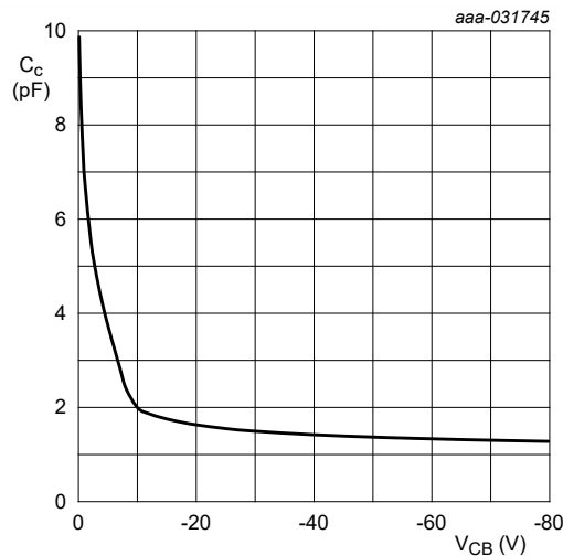
Fig. 9. NHDTA123JT: Collector capacitance as a function of collector-base voltage; typical values
