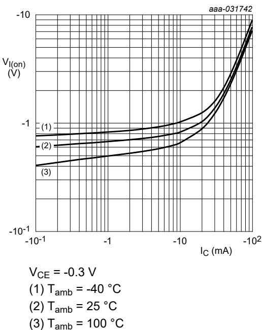
Fig. 6. NHDTA123JT: On-state input voltage as a function of collector current; typical values
