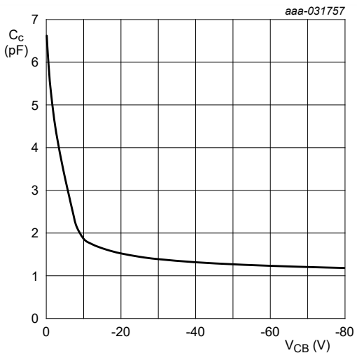
Fig. 21. NHDTA114YT: Collector capacitance as a function of collector-base voltage; typical values
