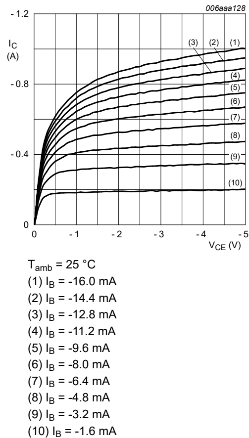
Fig. 5. BC807-16QB-Q: Collector current as a function of collector-emitter voltage; typical values
