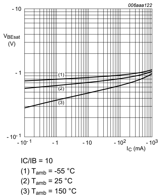
Fig. 6. BC807-16QB-Q: Base-emitter saturation voltage as a function of collector current; typical values
