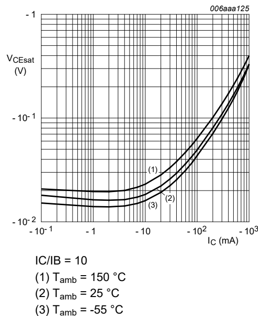
Fig. 7. BC807-16QB-Q: Collector-emitter saturation voltage as a function of collector current; typical values
