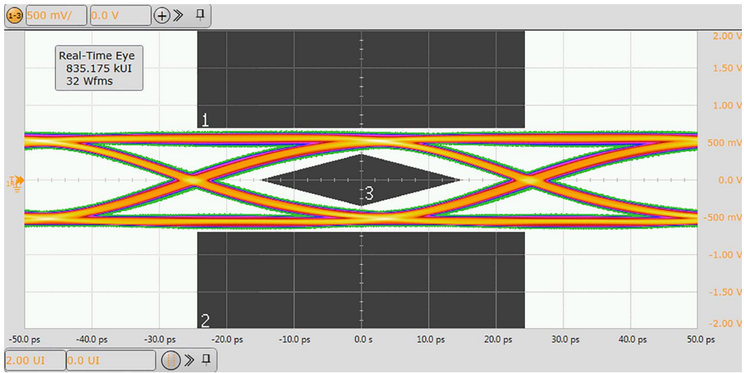
Fig. 12. Thunderbolt eye diagram, PCB with device; typical values
