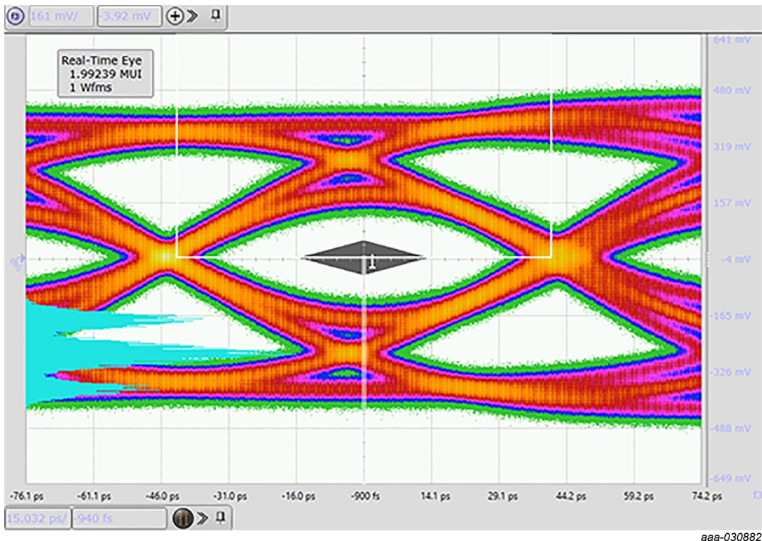
Fig. 11. HDMI 2.1 12G FRL TP2, Worst Case Model eye diagram, PCB without device; typical values
