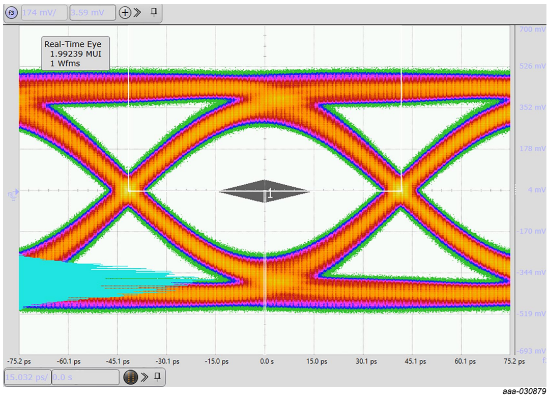
Fig. 8. HDMI 2.1 12G FRL TP1 eye diagram, PCB with device; typical values
