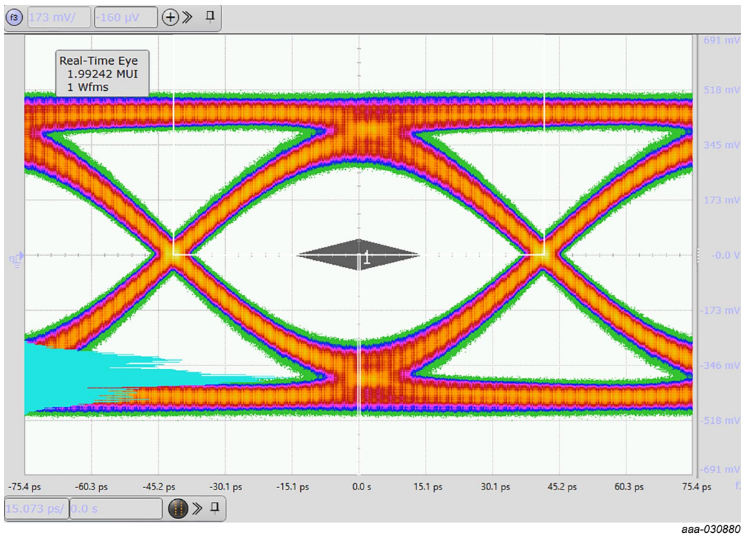
Fig. 9. HDMI 2.1 12G FRL TP1 eye diagram, PCB without device; typical values
