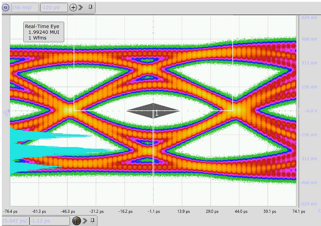
Fig. 10. HDMI 2.1 12G FRL TP2, Worst Case Model, 8 dB eye diagram, PCB with device; typical values
