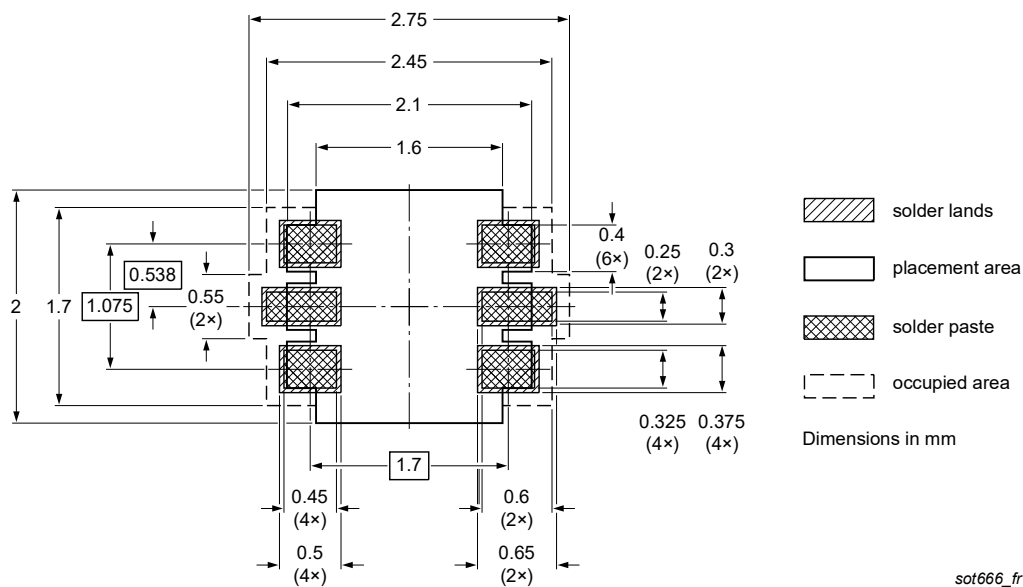
Fig. 4. Reflow soldering footprint for SOT666
