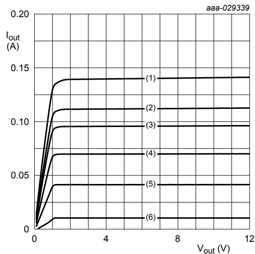
V_{EN} = 40\text{ V} ; T_{amb} = 25\text{ }^{\circ}\text{C} (1) R_{ext} = 6\text{ }\Omega (2) R_{ext} = 8\text{ }\Omega (3) R_{ext} = 10\text{ }\Omega (4) R_{ext} = 15\text{ }\Omega (5) R_{ext} = 30\text{ }\Omega (6) R_{ext} = \text{open}
