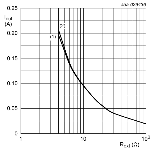
V_{EN} = 40\text{ V} ; T_{amb} = 25\text{ }^{\circ}\text{C} (1) V_{out} = 1.4\text{ V} (2) V_{out} = 5.4\text{ V}
