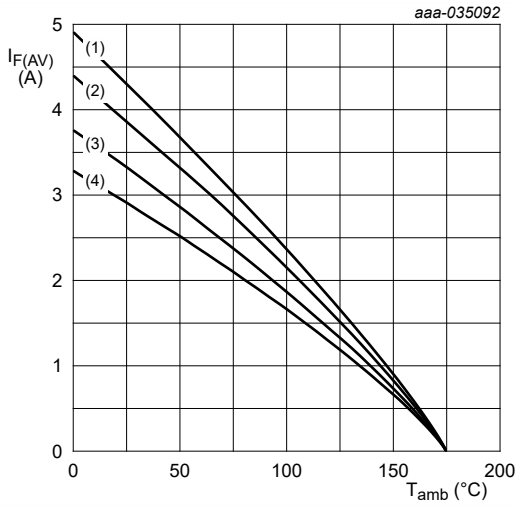
FR4 PCB, mounting pad for cathode 1 cm 2 T_j = 175 °C (1) \delta = 1 ; DC (2) \delta = 0.5 ; f = 20 kHz (3) \delta = 0.2 ; f = 20 kHz (4) \delta = 0.1 ; f = 20 kHz
