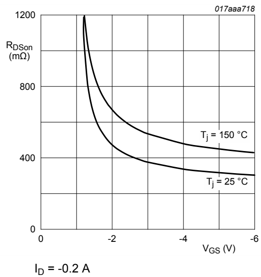
Fig. 10. Drain-source on-state resistance as a function of gate-source voltage; typical values I_D = -0.2\text{ A}
