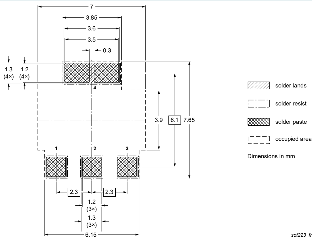
Fig. 20. Reflow soldering footprint for SC-73 (SOT223)
