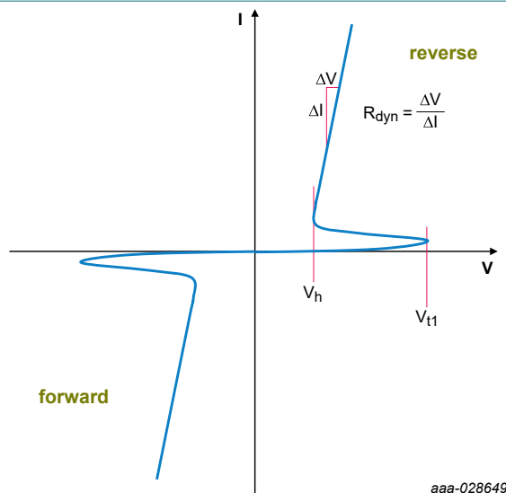
Fig. 9. Definition of snap-back voltage and trigger voltage in a Transmission Line Pulse (TLP) diagram
