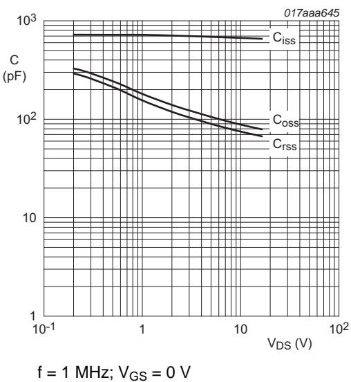
Fig 12. TR1: Input, output and reverse transfer capacitances as a function of drain-source voltage; typical values
