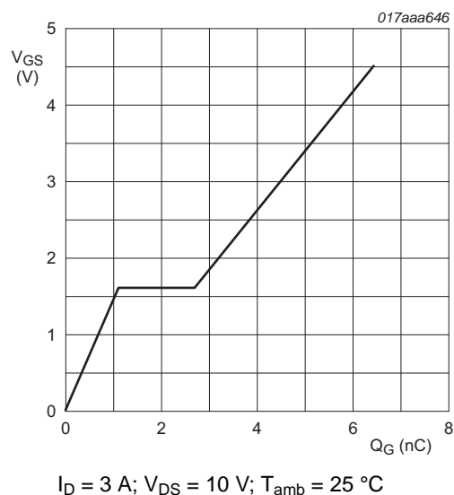
Fig 13. TR1: Gate-source voltage as a function of gate charge; typical values
