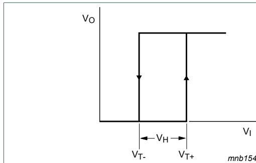
Fig. 6. Transfer characteristic
