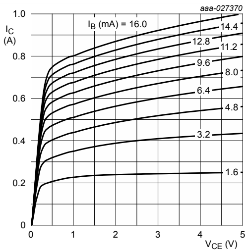
Figure 15. BC817K-16H: Collector current as a function of collector-emitter voltage; typical values
