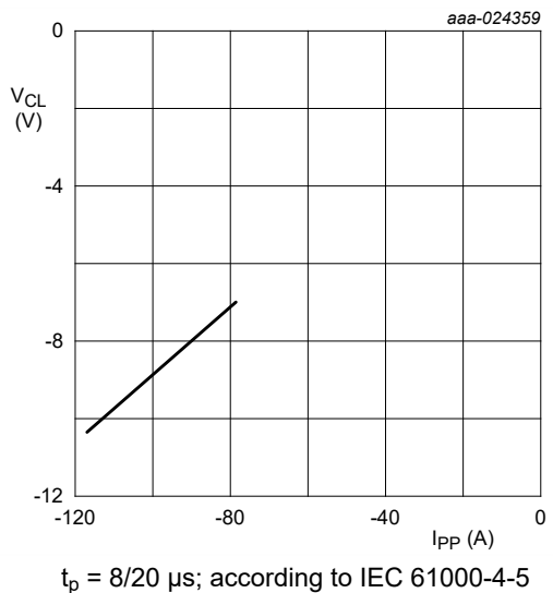
Fig. 11. Negative clamping voltage (8/20 \mu s pulse); typical values
