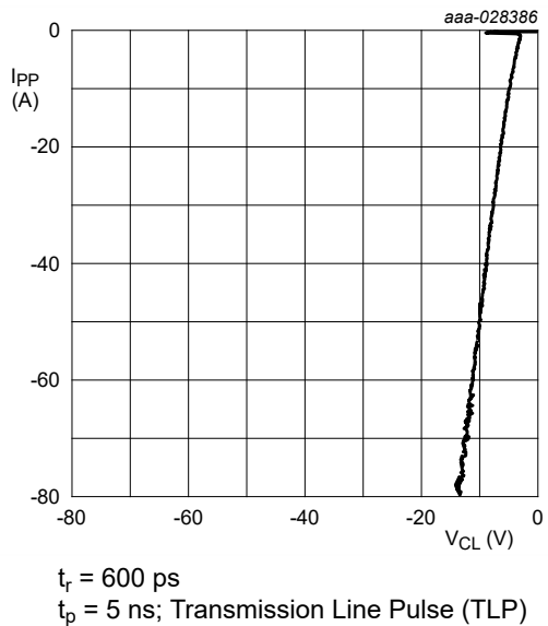
Fig. 17. Dynamic resistance with negative clamping; typical values
