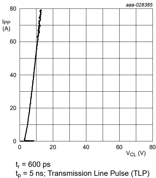
Fig. 16. Dynamic resistance with positive clamping; typical values
