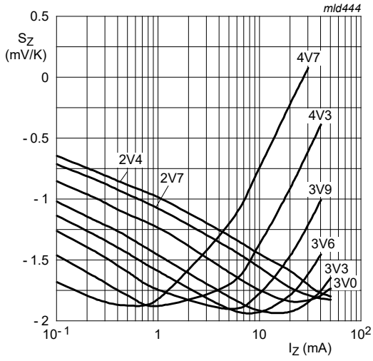
Fig. 5. Temperature coefficient as a function of working current; typical values (BZX884S-B/C2V4 to B/C4V7)
