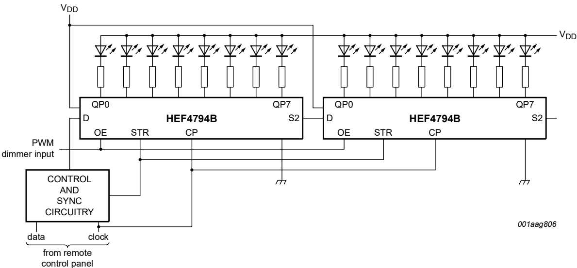
Fig. 10. Application example: serial-to-parallel data converting LED drivers
