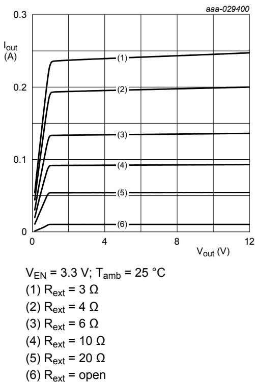
Fig. 16. NCR321Z: Output current as a function of output voltage; typical values
