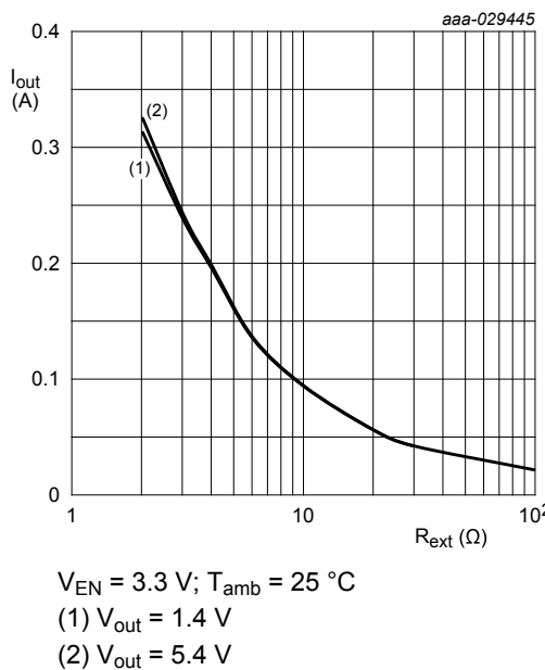
Fig. 17. NCR321Z: Output current as a function of external resistor; typical values
