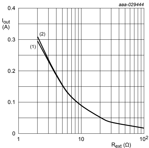
V_{EN} = 12\text{ V} ; T_{amb} = 25\text{ }^{\circ}\text{C} (1) V_{out} = 1.4\text{ V} (2) V_{out} = 5.4\text{ V}
