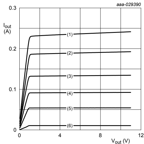
V_{EN} = 12\text{ V} ; T_{amb} = 25\text{ }^{\circ}\text{C} (1) R_{ext} = 3\text{ }\Omega (2) R_{ext} = 4\text{ }\Omega (3) R_{ext} = 6\text{ }\Omega (4) R_{ext} = 10\text{ }\Omega (5) R_{ext} = 20\text{ }\Omega (6) R_{ext} = \text{open}
