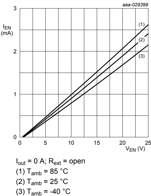
Fig. 15. NCR320Z: Enable current as a function of enable voltage; typical values
