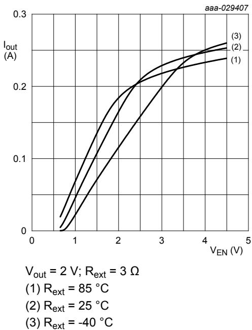
Fig. 23. NCR321Z: Output current as a function of enable voltage; typical values
