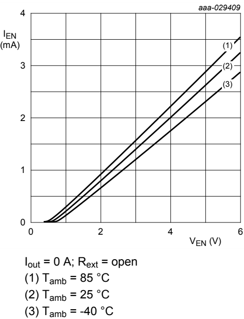
Fig. 25. NCR321Z: Enable current as a function of enable voltage; typical values
