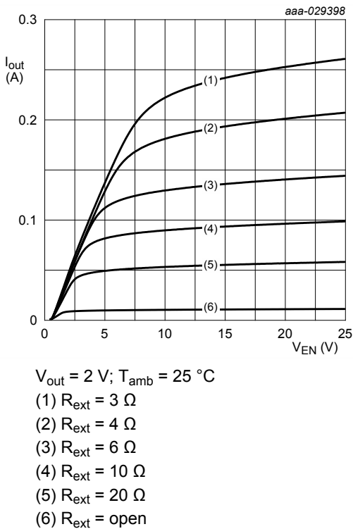
Fig. 14. NCR320Z: Output current as a function of enable voltage; typical values
