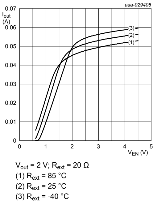
Fig. 22. NCR321Z: Output current as a function of enable voltage; typical values
