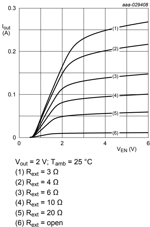
Fig. 24. NCR321Z: Output current as a function of enable voltage; typical values
