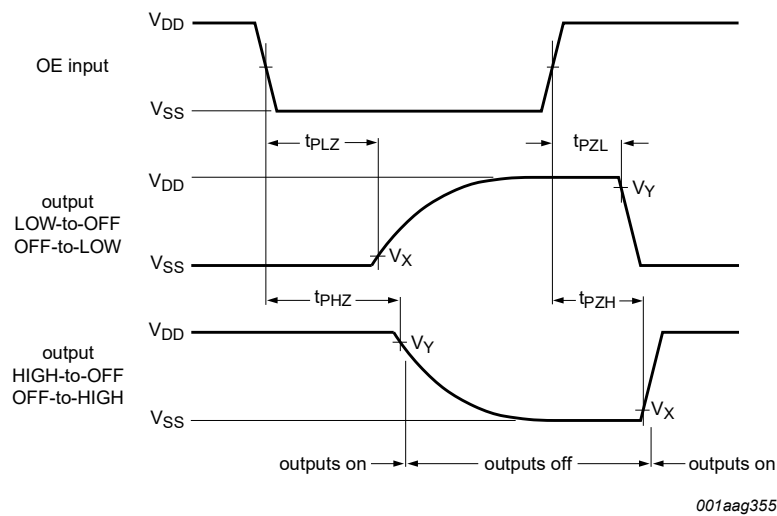
Fig. 5. Output enable (OE) to latch output (nQ) enable time ( t_{PZH} and t_{PZL} ) and disable time ( t_{PLZ} and t_{PHZ} )
