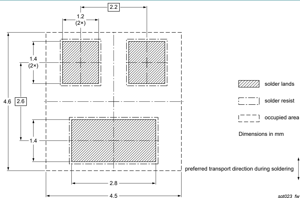
Fig. 12. Wave soldering footprint for SOT23
