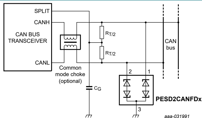
Fig. 8. Typical application: ESD protection of two automotive CAN bus lines
