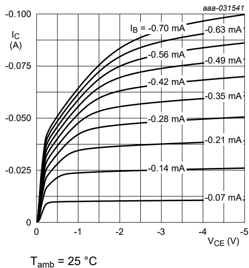
Fig. 10. NHUMB11: Collector current as a function of collector-emitter voltage; typical values
