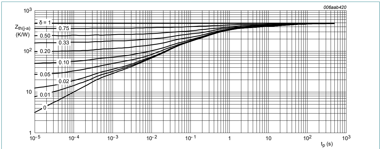
FR4 PCB, single-sided, 35 µm copper, tin-plated and standard footprint
