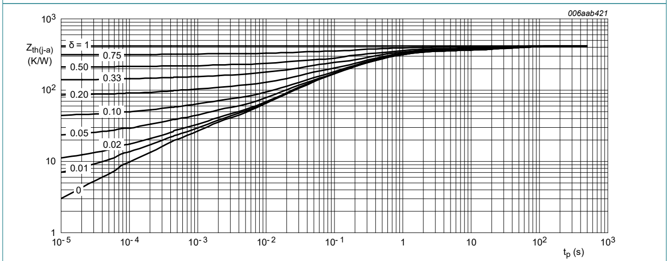
FR4 PCB, single-sided, 35 µm copper, tin-plated, mounting pad for collector 1 cm 2
