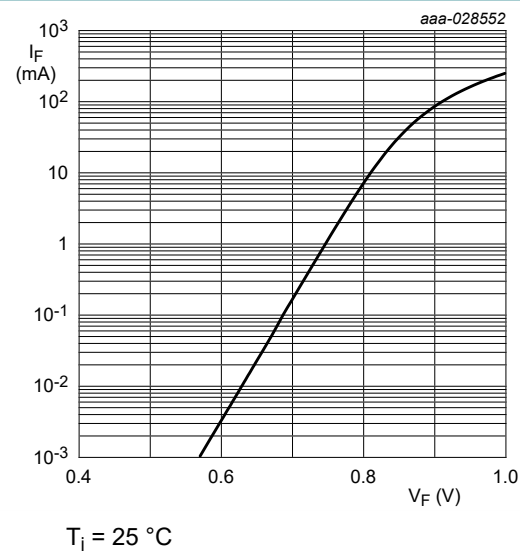
Fig. 4. Per diode: Forward current as a function of forward voltage; typical values (BZB84-B/C7V5-Q)
