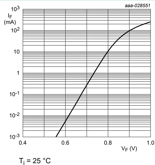
Fig. 3. Per diode: Forward current as a function of forward voltage; typical values (BZB84-B/C6V8-Q)
