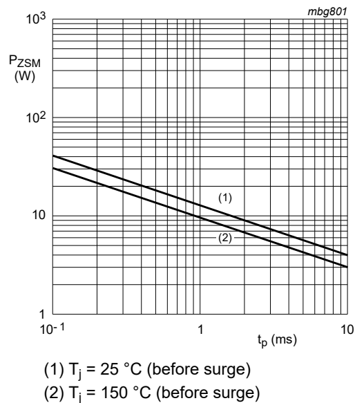
Fig. 1. Per diode: Non-repetitive peak reverse power dissipation as a function of pulse duration; maximum values
