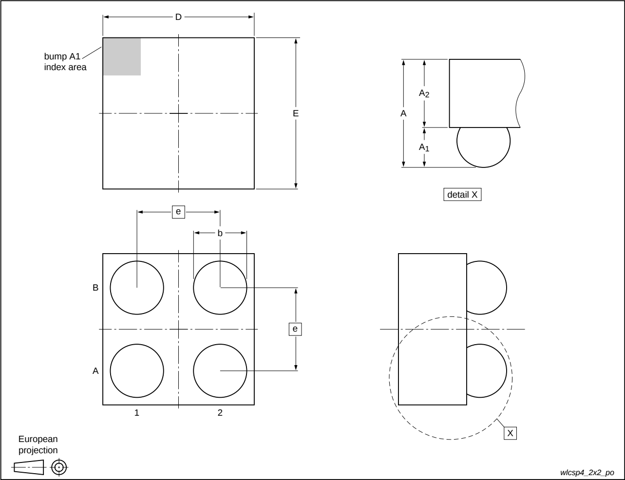
WLCSP4: wafer level chip-size package; 4 bumps (2 x 2)
