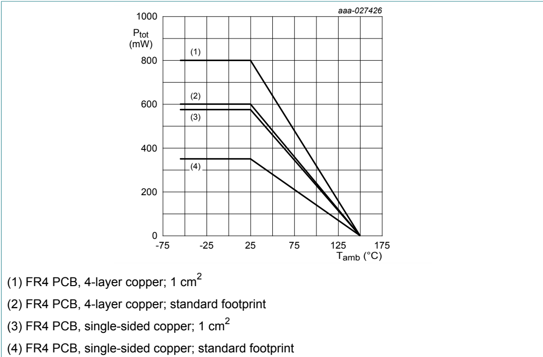
Figure 1. Power derating curves
