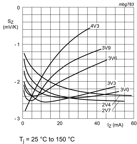
Fig. 6. Temperature coefficient as a function of working current; typical values (BZT52-B2V4 to BZT52-B4V3)
