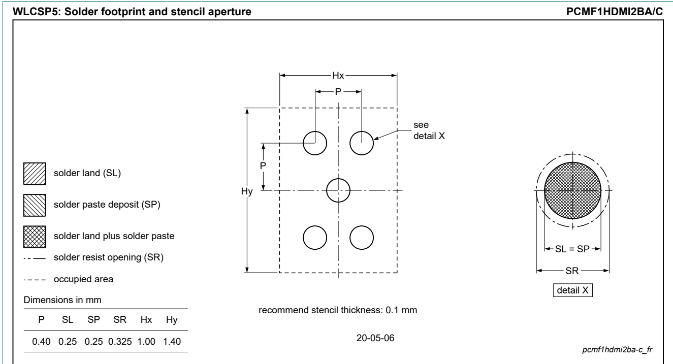
Fig. 20. Soldering footprint WLCSP5 (PCMF1HDMI2BA/C)
