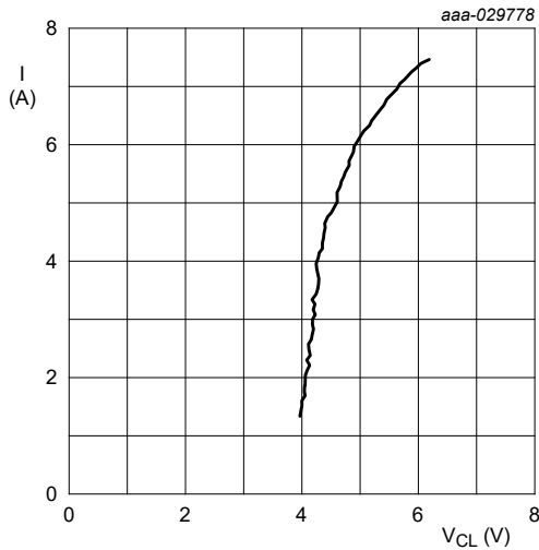
Fig. 15. Dynamic resistance with positive clamping; typical values
