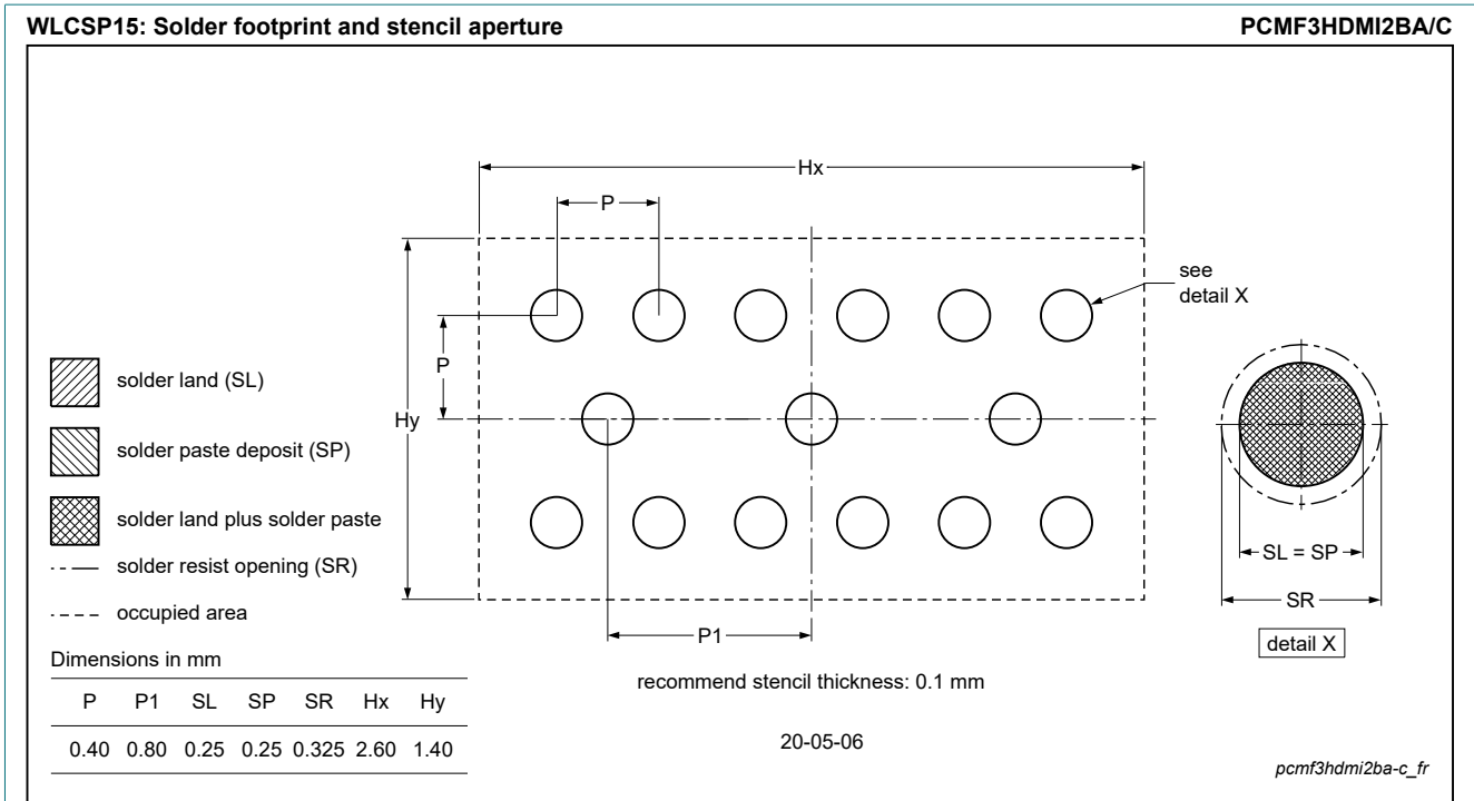
Fig. 22. Soldering footprint WLCSP15 (PCMF3HDMI2BA/C)
