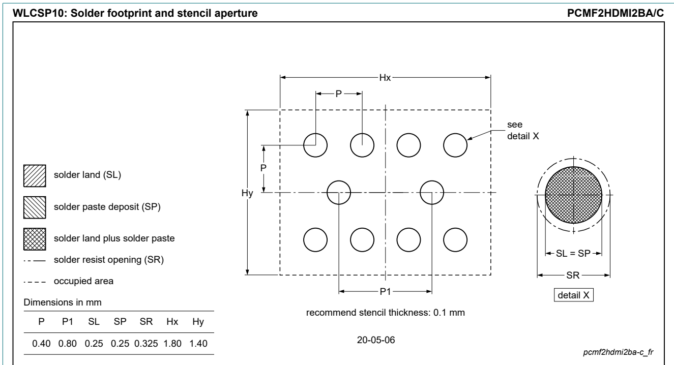
Fig. 21. Soldering footprint WLCSP10 (PCMF2HDMI2BA/C)
