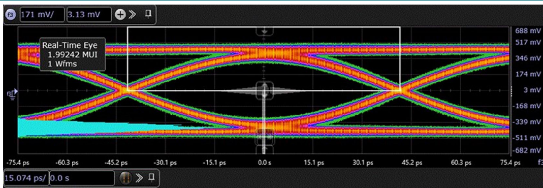
Fig. 5. HDMI 2.1 12G FRL eye diagram, PCB with device; typical values
