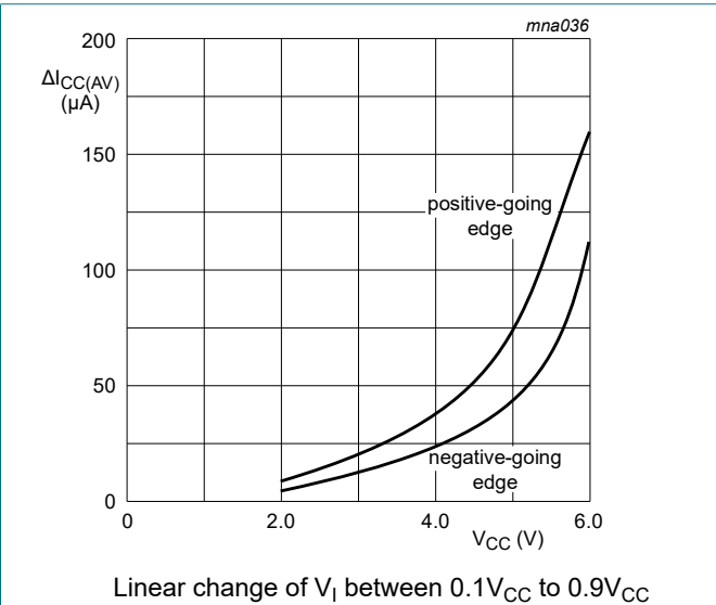
Fig. 13. Average additional I_{CC} for 74AHC3G14-Q100 Schmitt trigger devices
