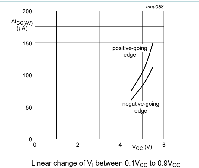
Fig. 14. Average additional I_{CC} for 74AHCT3G14-Q100 Schmitt trigger devices
