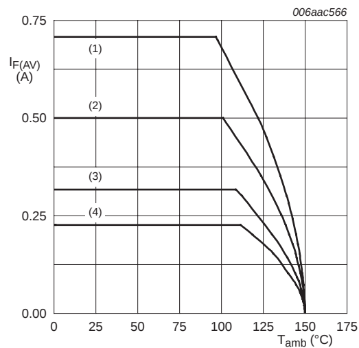
FR4 PCB, mounting pad for cathode 1 cm² T_j = 150 °C (1) \delta = 1 ; DC (2) \delta = 0.5 ; f = 20 kHz (3) \delta = 0.2 ; f = 20 kHz (4) \delta = 0.1 ; f = 20 kHz
