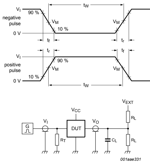
Test data is given in Table 9 . All input pulses are supplied by generators having the following characteristics: PRR \leq 10\text{ MHz} ; Z_o = 50\ \Omega . The outputs are measured one at a time with one transition per measurement. Definitions for test circuit: R_L = Load resistance. C_L = Load capacitance including jig and probe capacitance. R_T = Termination resistance should be equal to output impedance Z_o of the pulse generator. V_{EXT} = External voltage for measuring switching times.
