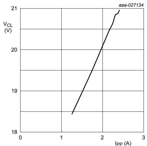
Fig. 10. Positive clamping voltage (10/1000 \mu s pulse); typical values
