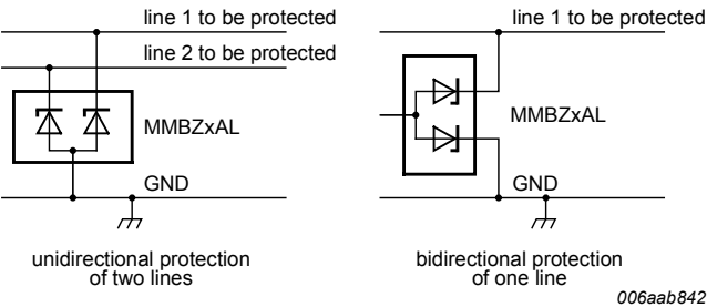
Fig. 15. Application diagram
