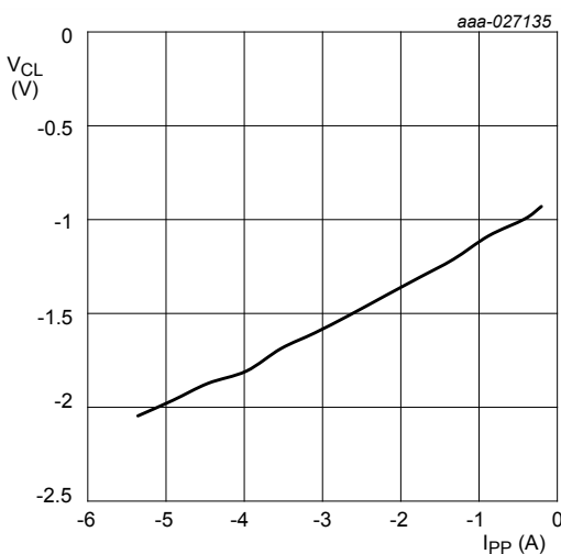
Fig. 11. Negative clamping voltage (10/1000 \mu s pulse); typical values
