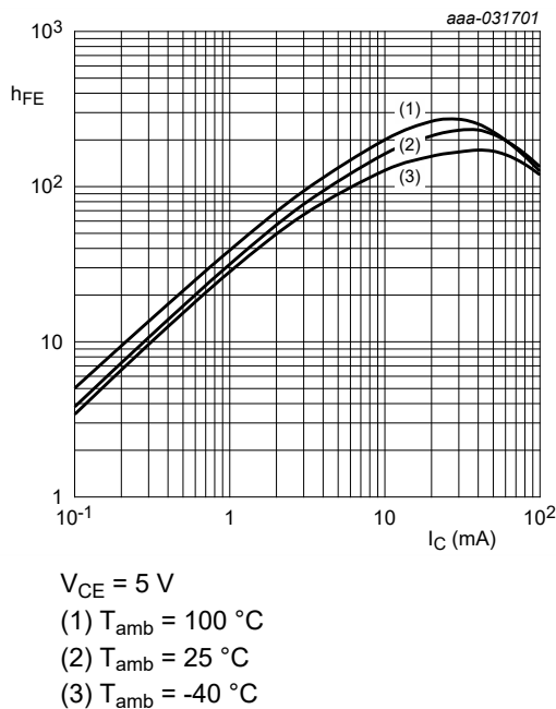
Fig. 9. NHUMH11: DC current gain as a function of collector current; typical values
