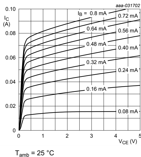
Fig. 10. NHUMH11: Collector current as a function of collector-emitter voltage; typical values
