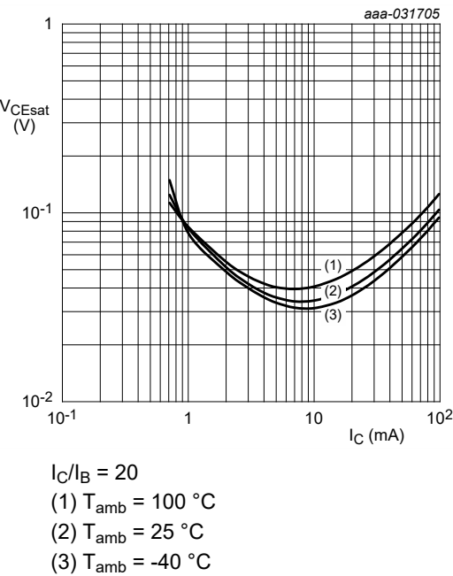
Fig. 13. NHUMH1: Collector-emitter saturation voltage as a function of collector current; typical values
