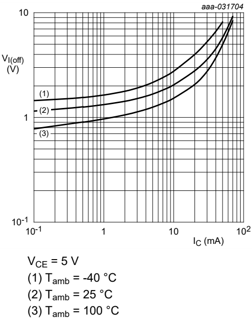
Fig. 12. NHUMH1: Off-state input voltage as a function of collector current; typical values
