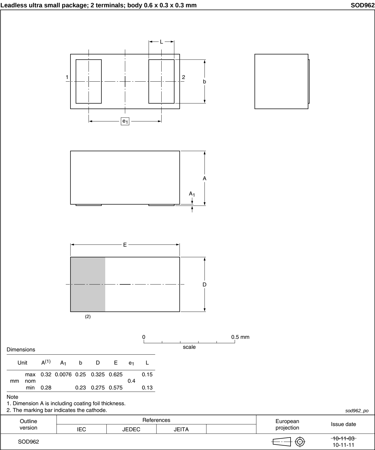
Fig 11. Package outline PESD5V0L1BSF (SOD962)
