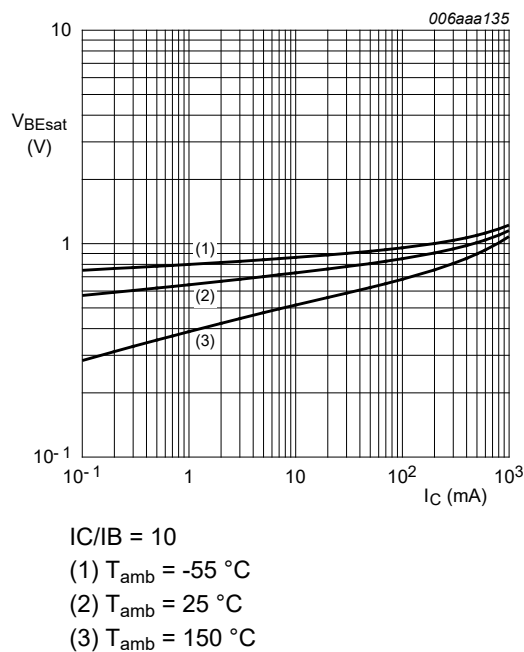
Fig. 10. BC817-25QBH-Q: Base-emitter saturation voltage as a function of collector current; typical values
