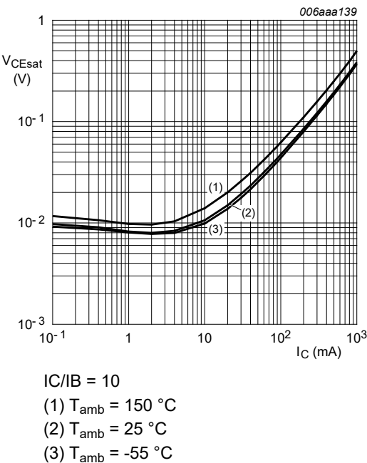
Fig. 15. BC817-40QBH-Q: Collector-emitter saturation voltage as a function of collector current; typical values
