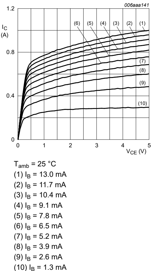
Fig. 9. BC817-25QBH-Q: Collector current as a function of collector-emitter voltage; typical values
