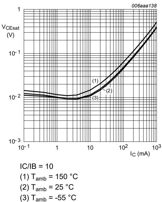
Fig. 11. BC817-25QBH-Q: Collector-emitter saturation voltage as a function of collector current; typical values
