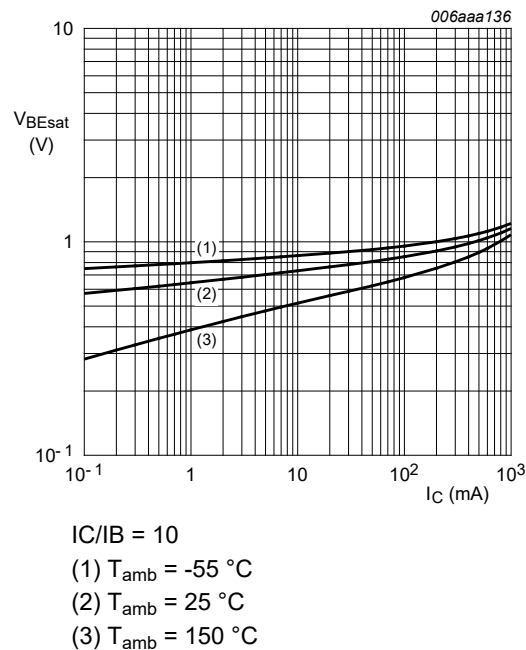
Fig. 14. BC817-40QBH-Q: Base-emitter saturation voltage as a function of collector current; typical values
