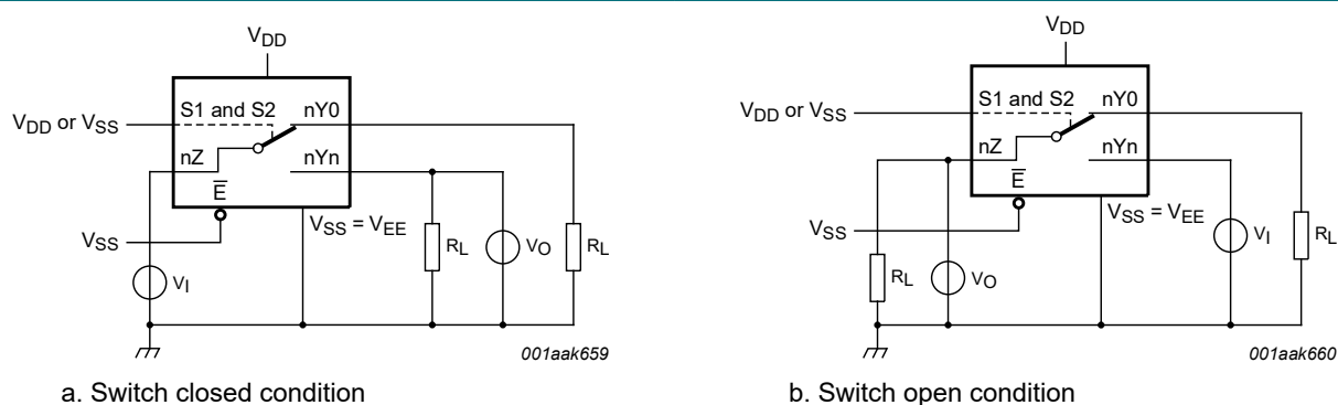
Fig. 21. Test circuit for measuring crosstalk between switches
