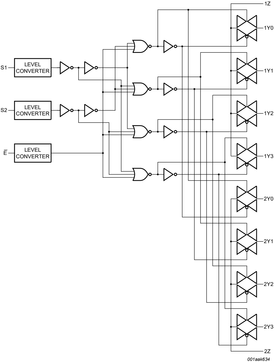
Fig. 5. Logic diagram
