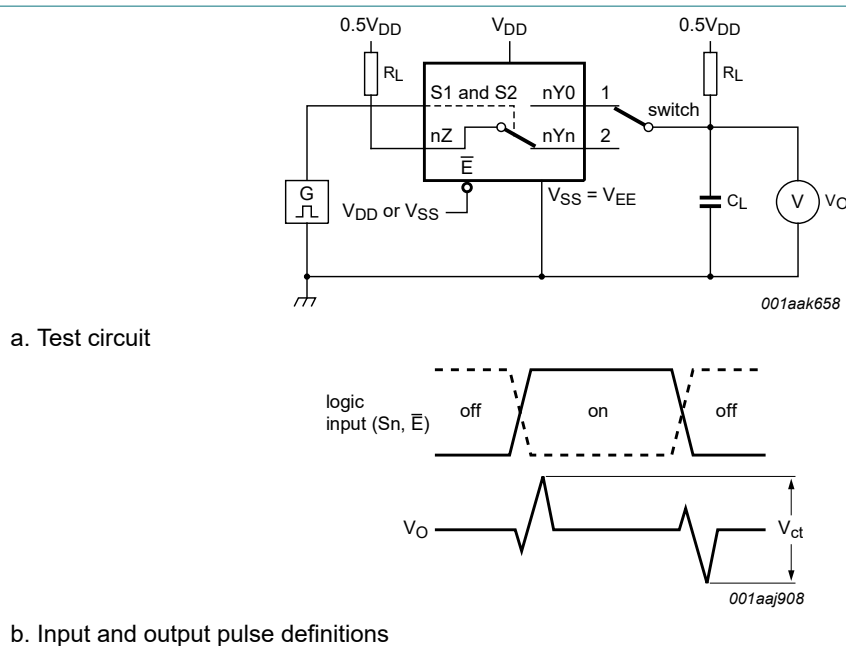
Fig. 20. Test circuit for measuring crosstalk voltage between digital inputs and switch
