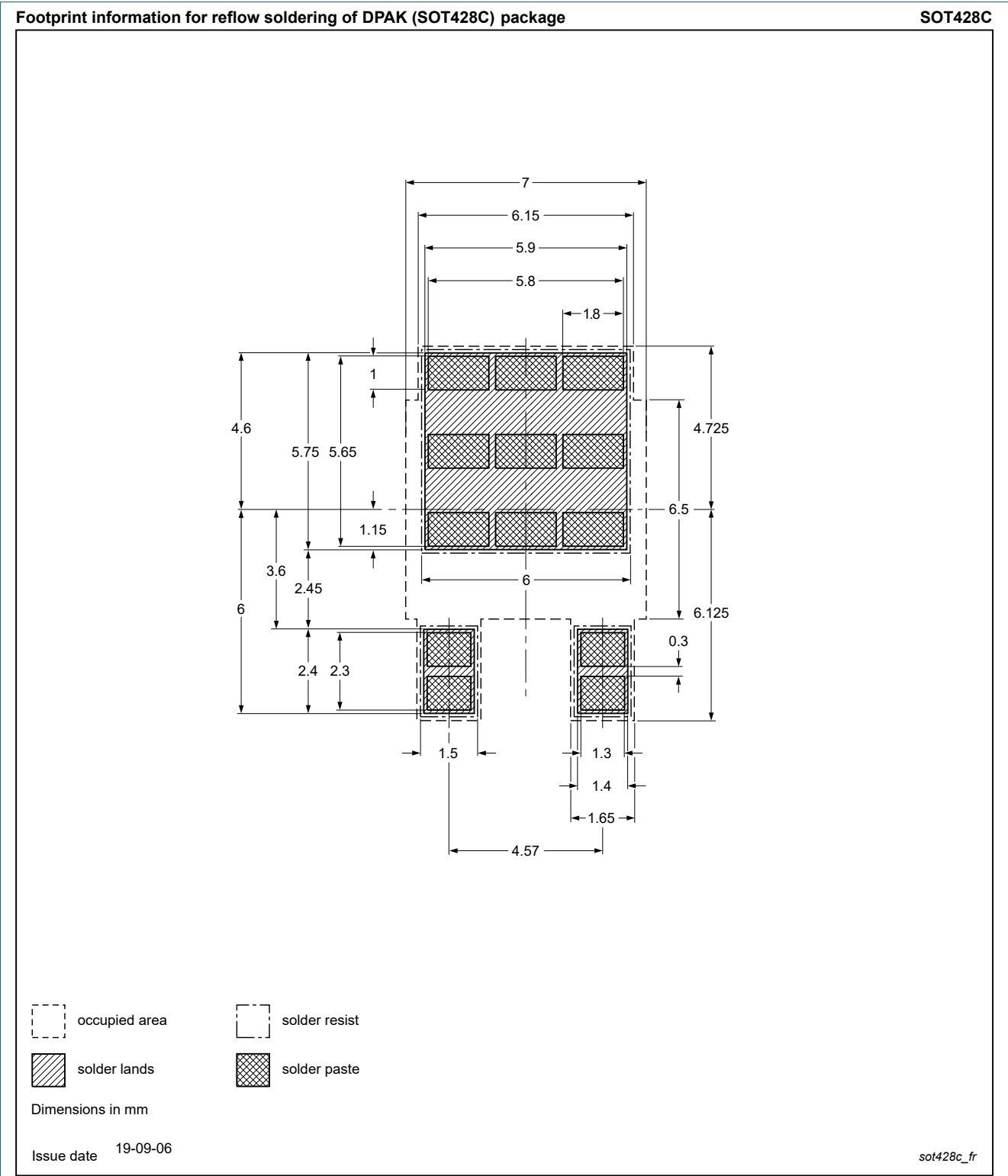
Fig. 13. Reflow soldering footprint for DPAK (SOT428C)
