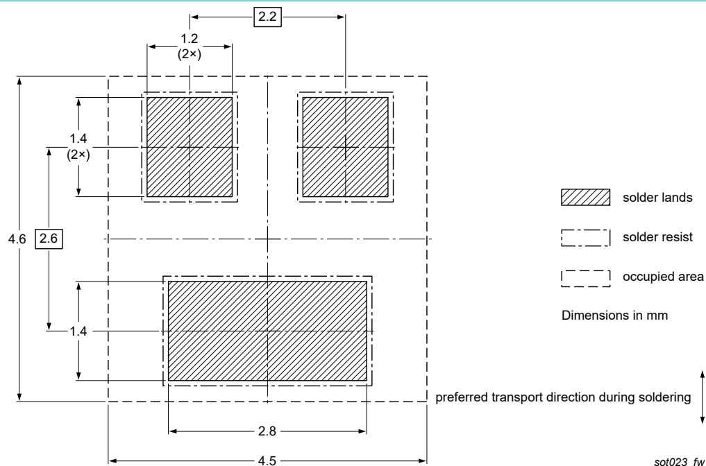
Fig. 15. Wave soldering footprint for SOT23
